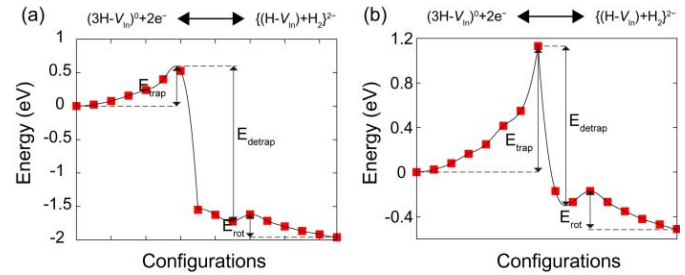
Fig. 8. Calculated configuration coordination diagram describing the transformation from (3H - V_{In})^0 into \{(H - V_{In}) + H_2\}^{2-} . (a) E_F = E_{CB} + 0.74 eV and (b) E_F = E_{CB} + 0.21 eV. E_{trap} and E_{detrapp} are the energy barriers for electron trap and detrapp process, respectively. E_{rot} is the activation energy for the rotation of H_2 molecule.
