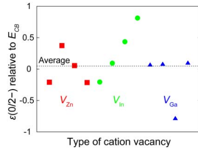
Fig. 7. Transition levels, \epsilon(0/2-) . Corresponding to the E_F level at which \{(N - 2)H - V_M + H_2\}^{2-} begins to be more stable than (NH - V_M)^0 .
