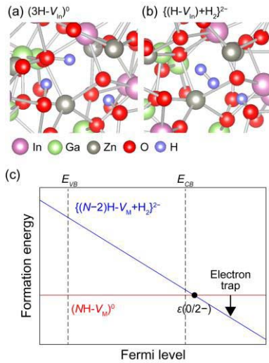
Fig. 6. (NH - V_M)^0 different atomic configurations state. (a) Atomic structures of (NH - V_M)^0 for M = \text{In} . (b) Electrons can lead to the binding between neighboring hydrogen ions, i.e., 2H^+ + 2e^- \rightarrow H_2 , which transforms (NH - V_M)^0 into \{(N - 2)H - V_M + H_2\}^{2-} . (c) Change of the formation energies of (NH - V_M)^0 and \{(N - 2)H - V_M + H_2\}^{2-} .
